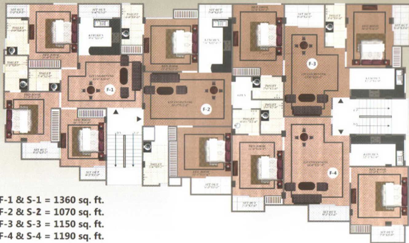
First Floor Plan Second Floor Plan
